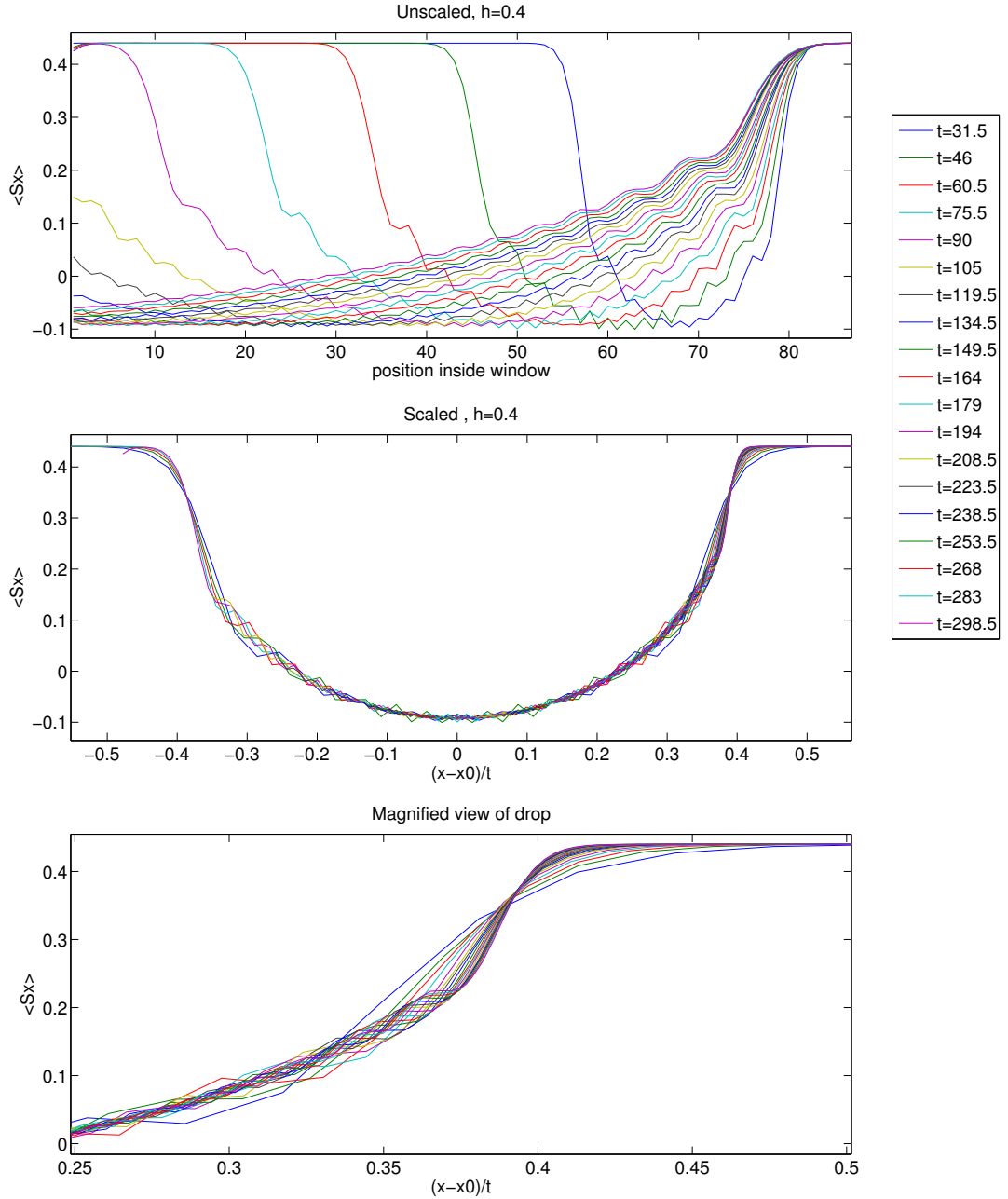
Figure 6.22.: Magnetization time slices in x of a spin flip in x on the TIM for h = 0.4 . The top panel shows the unscaled magnetizations time slices at different times, the horizontal axis marks position inside the CMW. The middle panel shows the rescaled time slices, where the position axis has been scaled according to (6.10) with x_0 = \frac{L}{2} . Whereas the general shape, as well as the total width of the signal scale linearly with time and thus overlap well, the characteristic drops at the light cone boundaries do not. They vary over time in scaled width and magnitude. The bottom panel shows a magnified view of the characteristic drops.
