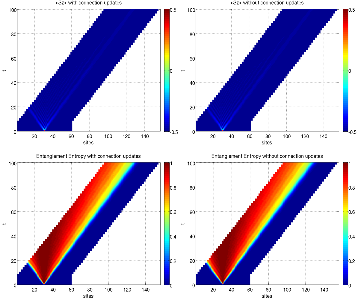
Figure 6.3.: Single magnon excitation of the XX chain for J = 1 with \tau = 0.01 and m = 8 . The timelines for the magnetization \langle \hat{S}_j^z(t) \rangle and bipartite entanglement entropy S_{ent}(t) (cf. (3.40)) for the simulations with (on the left) and without connection updates (on the right) show no significant difference. Largest deviations are of the order \mathcal{O}(10^{-5}) at the point, where the left signal branch hits the rear boundary. This is due to the switch to obc for the simulation using connection updates.
