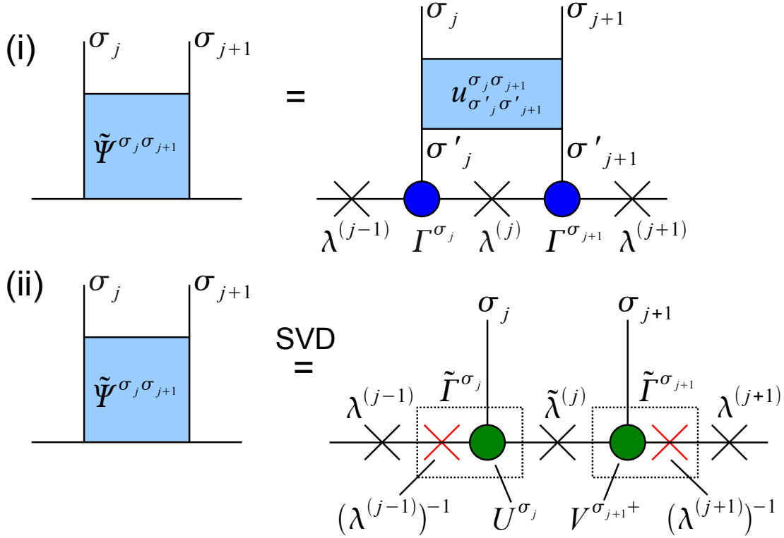
Figure 4.7.: TEBD update for a single bond. (i) Form the 2-site wave function \Psi^{\sigma_j \sigma_{j+1}} and apply the 2-site time evolution operator u_{\sigma'_j \sigma'_{j+1}}^{\sigma_j \sigma_{j+1}} to get \tilde{\Psi}^{\sigma_j \sigma_{j+1}} . (ii) Decompose via SVD to get \tilde{\Psi}^{\sigma_j \sigma_{j+1}} = U^{\sigma_j} \tilde{\lambda}^{(j)} V^{\sigma_{j+1} \dagger} and extract updated \tilde{\lambda}^{(j)} , \tilde{\Gamma}^{\sigma_j} and \tilde{\Gamma}^{\sigma_{j+1}} using (4.54) and (4.55).
